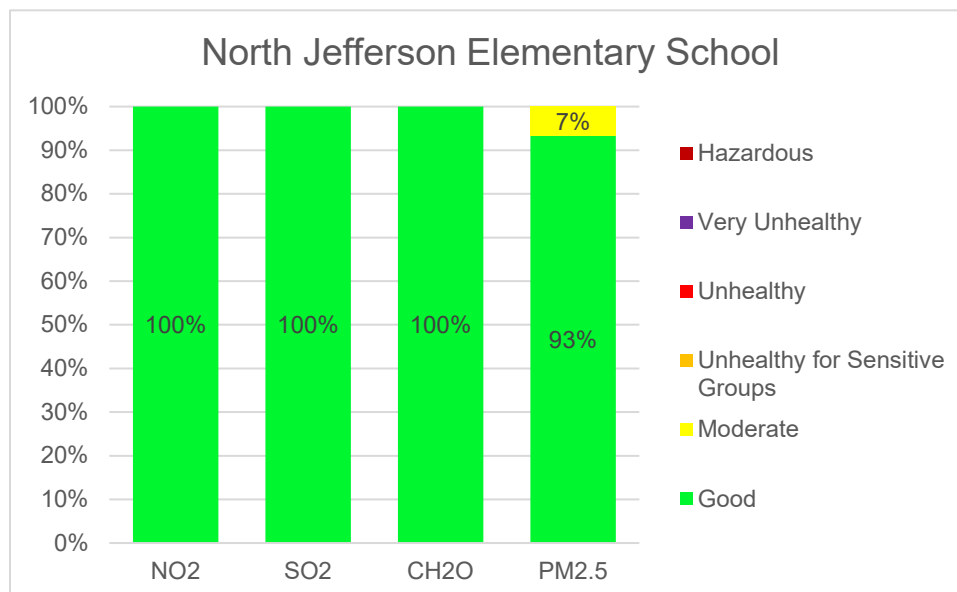
Figure 7: NJES AQI Distribution Summary — July through September 2022
