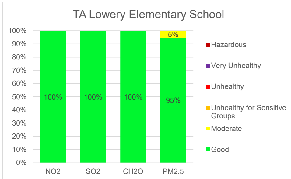
Figure 2: TALES AQI Distribution Summary — July through September 2022
