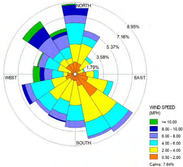
Figure 11: September 2022 Wind Rose
