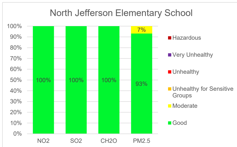
Figure 1: NJES AQI Distribution Summary — July through September 2022
