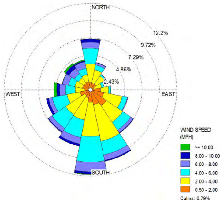
Figure 12: July through September 2022 Wind Rose
