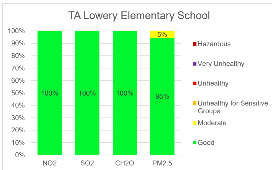
Figure 8: TALES AQI Distribution Summary — July through September 2022
