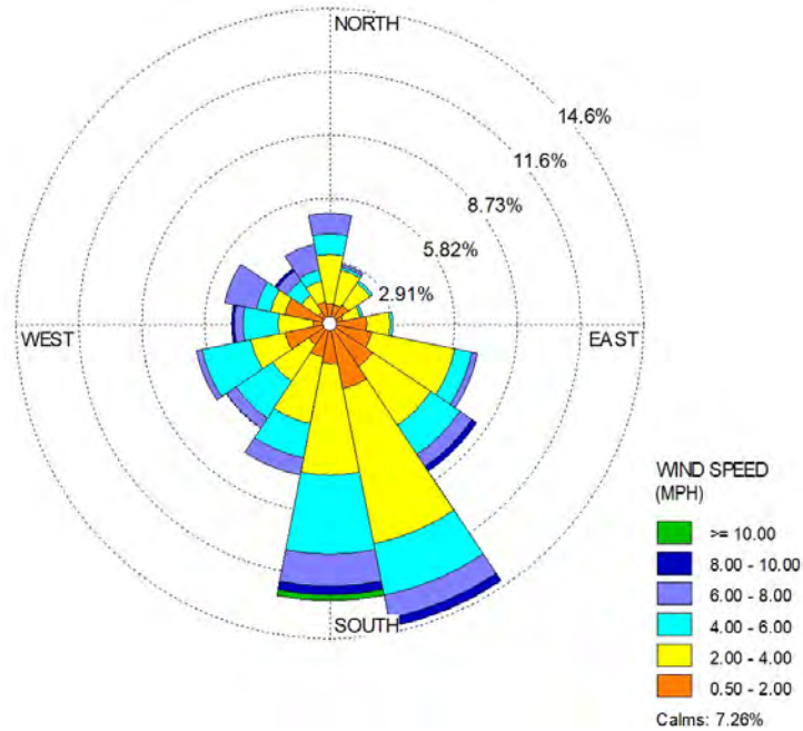
Figure 10: August 2022 Wind Rose
