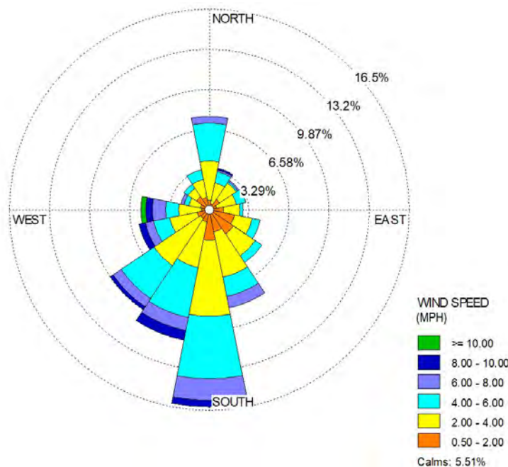
Figure 9: July 2022 Wind Rose
